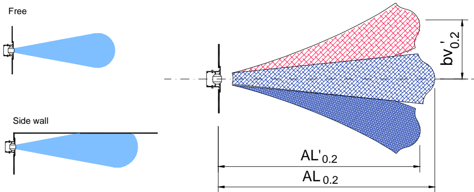
CORRECTION FACTOR FOR THROW (L0.2) DT (-).
