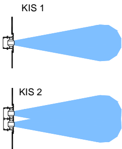
CORRECTION FACTOR FOR THROW KL
