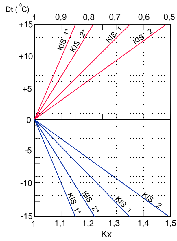
CORRECTION FACTOR FOR VERTICAL THROW ( AV_{0,2} ) DT
