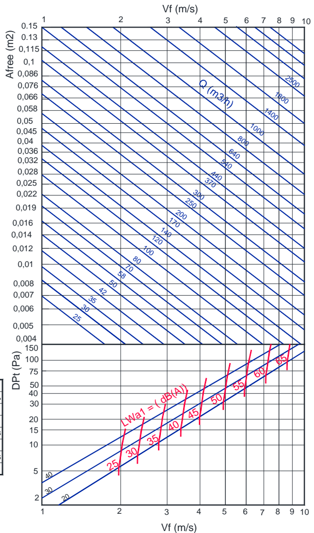
FREE VELOCITY, PRESSURE LOSS AND SOUND POWER LEVEL.
